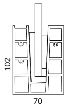
ENDCAP
