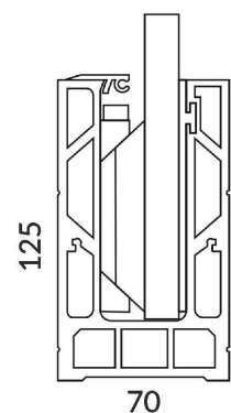
ENDCAP
