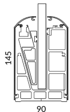
ENDCAP
