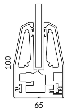
ENDCAP
