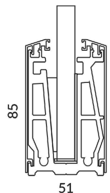
ENDCAP
