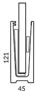
ENDCAP
